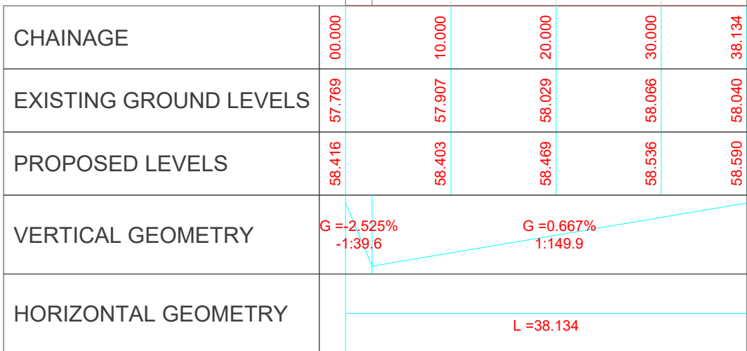
ROAD 02.1 LONGSECTION SCALE: H 1:500, V 1:100. DATUM: 55.000
