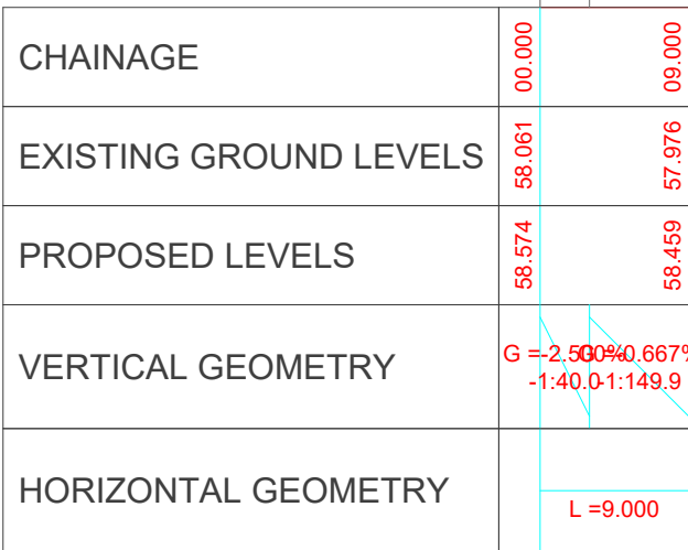
ROAD 02.1.1 LONGSECTION SCALE: H 1:500, V 1:100. DATUM: 55.000
