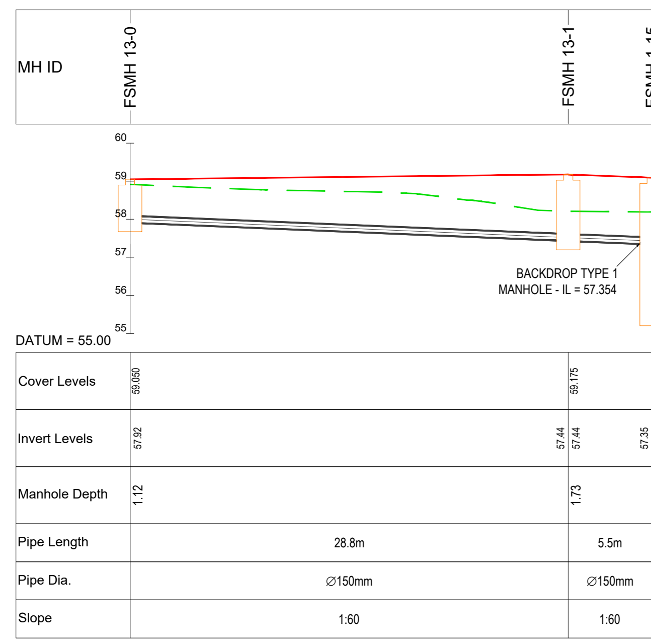
FSMH 13-0 TO FSMH 1-15 - PROFILE SCALE: H 1:250, V 1:100
