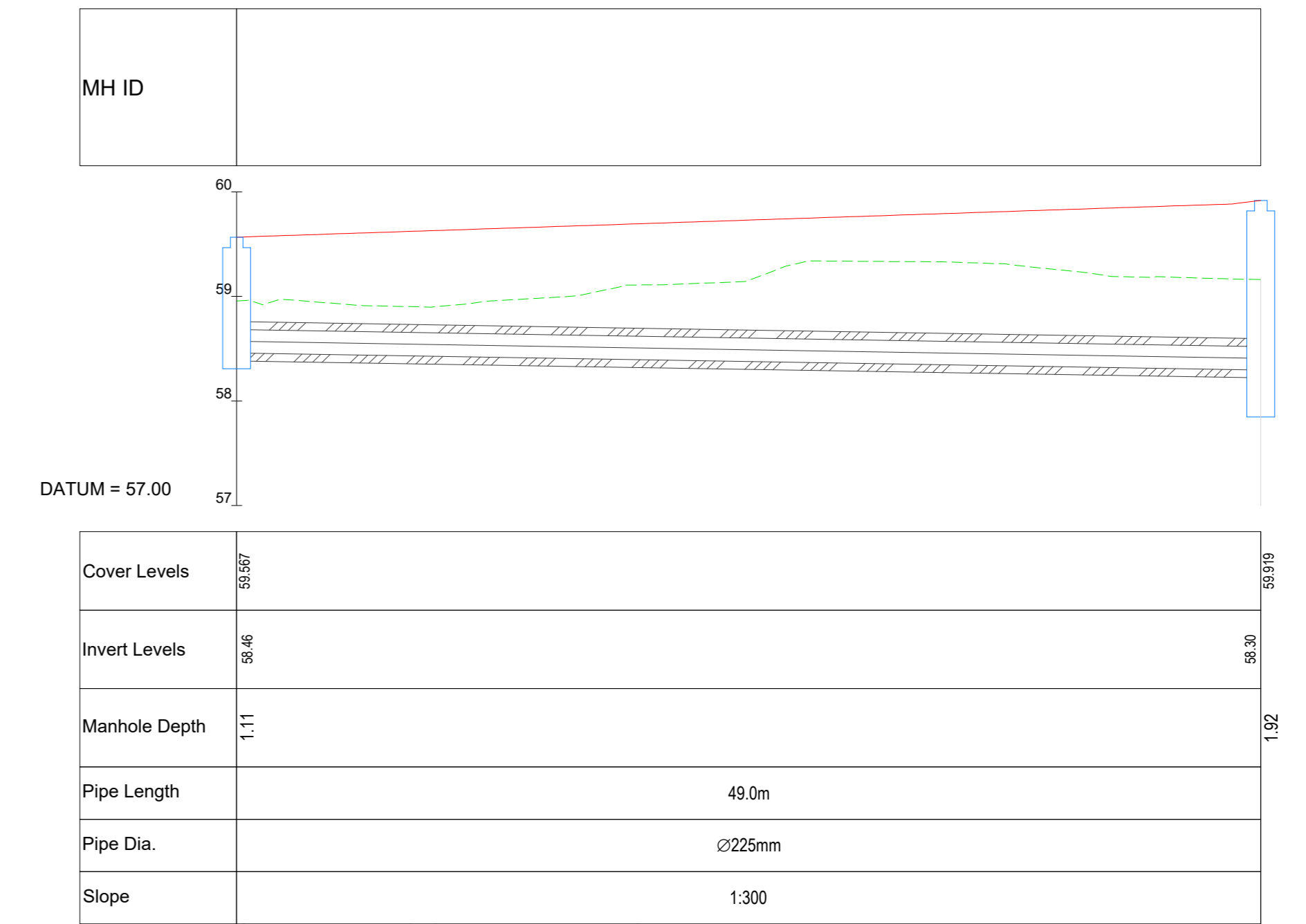
SWMH 6E-0 TO SWMH 6B-2 - PROFILE SCALE: H 1:250, V 1:50
