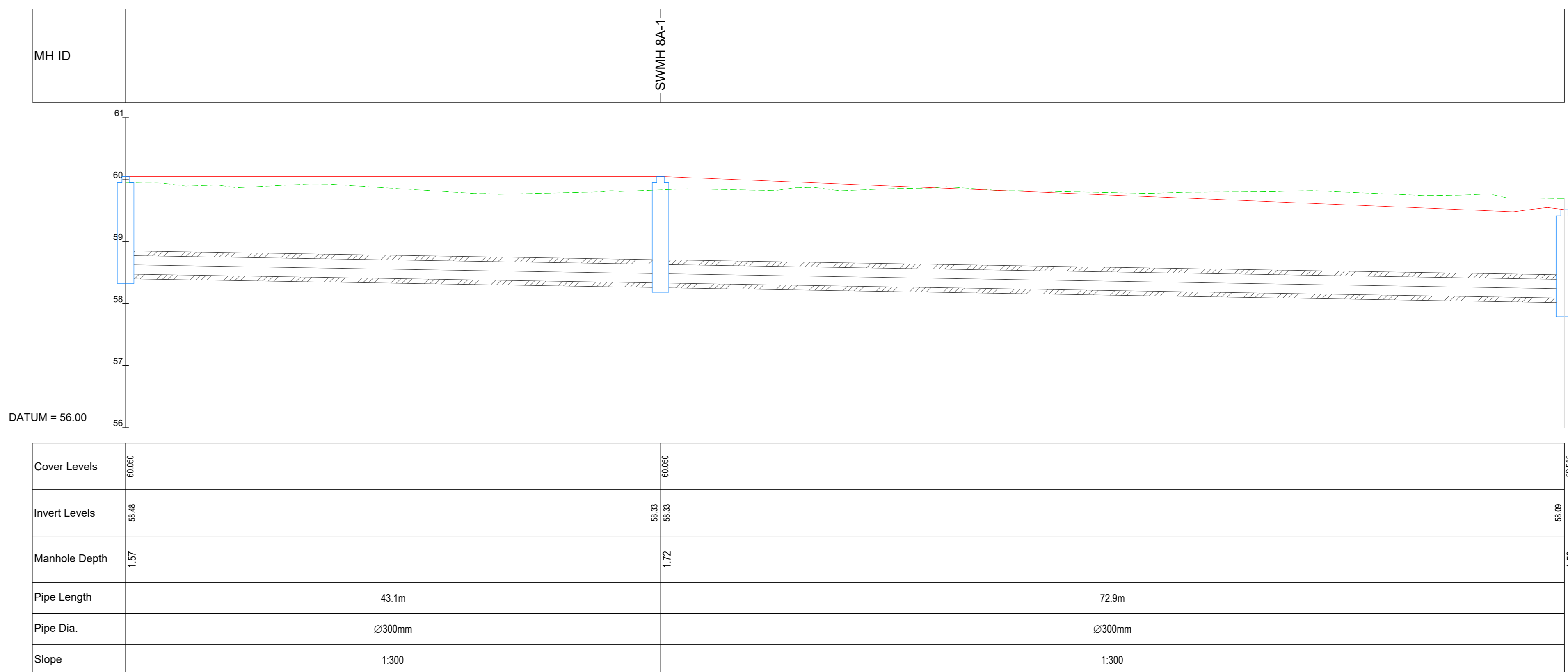
SWMH 8A-0 TO SWMH 8-3 - PROFILE SCALE: H 1:250, V 1:50
