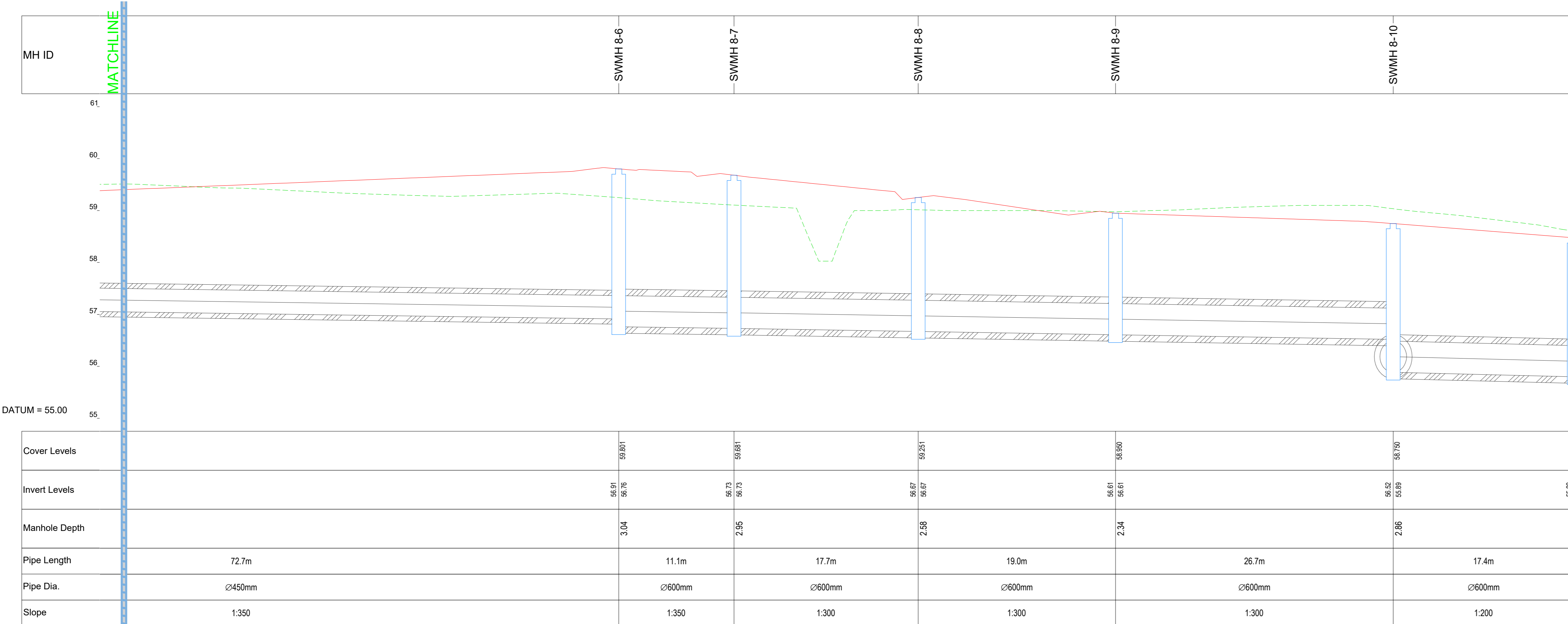
SWMH 8-0 TO SWMH 8-11 - PROFILE SCALE: H 1:250, V 1:50
