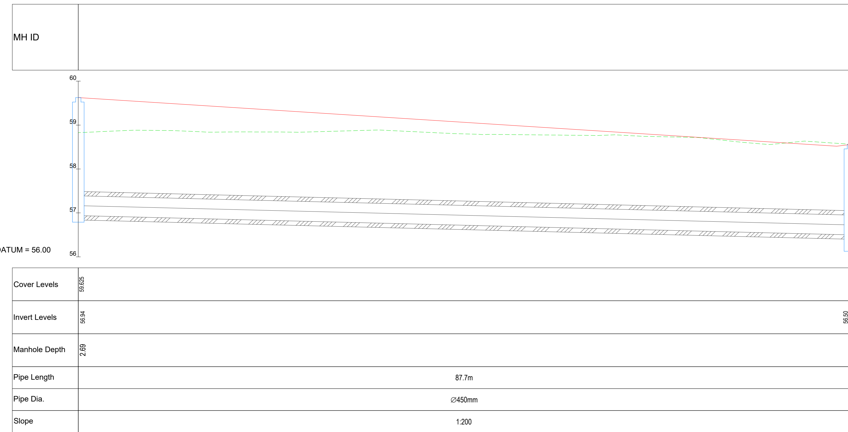
SWMH 7H-0 TO SWMH 7-16 - PROFILE SCALE: H 1:250, V 1:50
