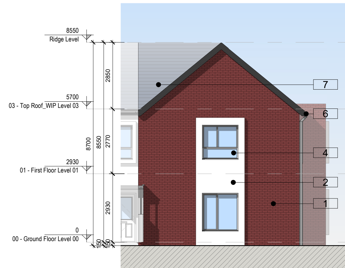
4 SIDE ELEVATION 1 : 100
