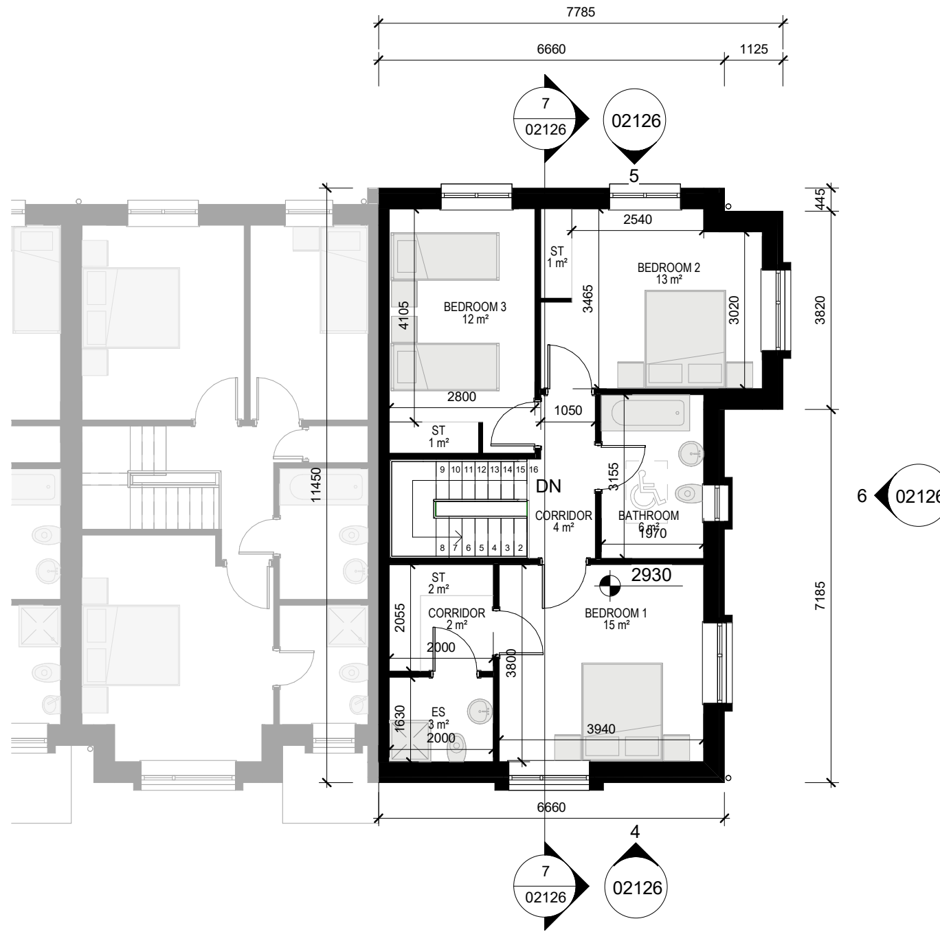
2 FIRST FLOOR PLAN 1 : 100
