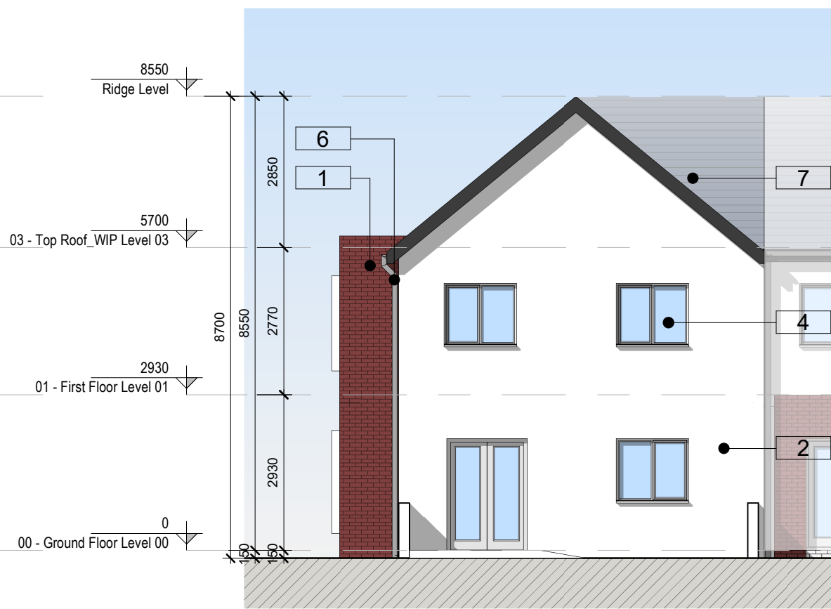
5 SIDE ELEVATION 1 : 100
