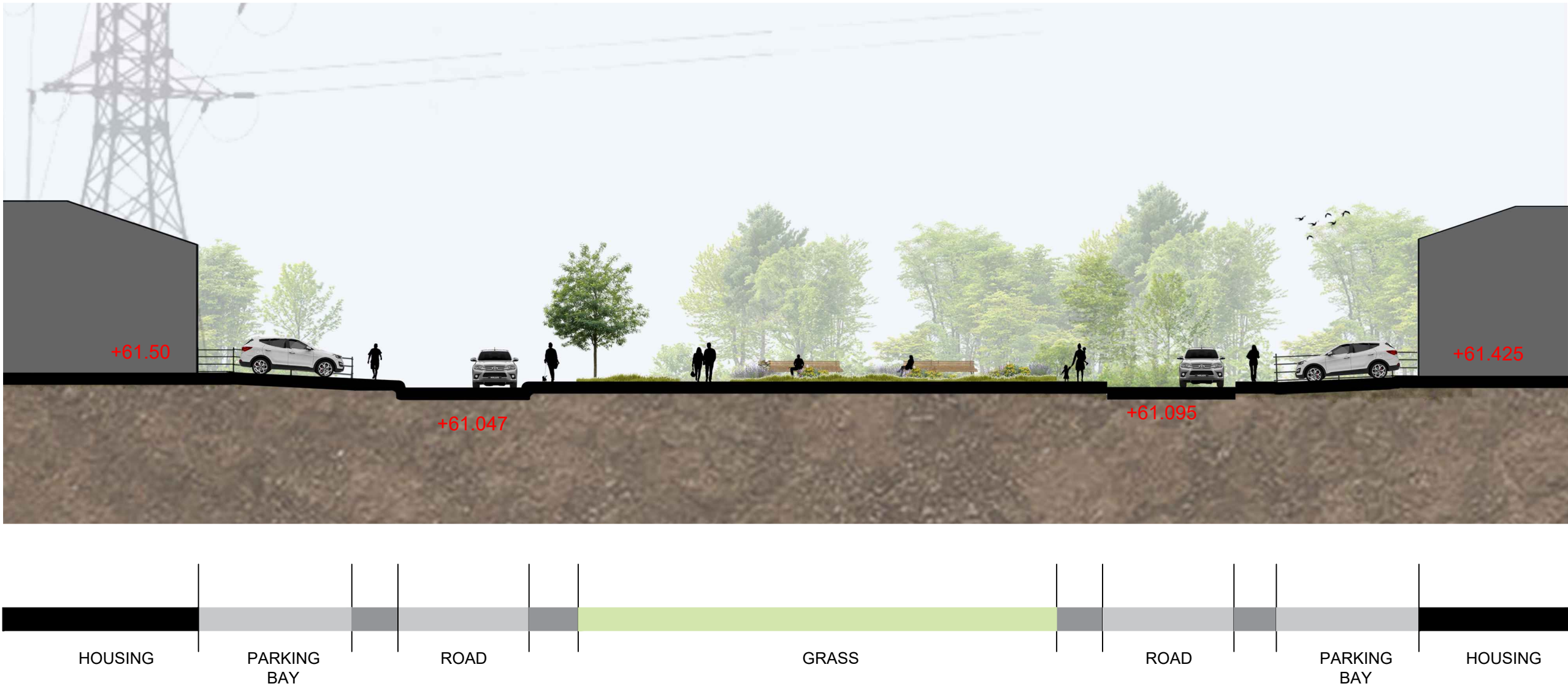
LANDSCAPE SECTION 15-15 sc 1/200
