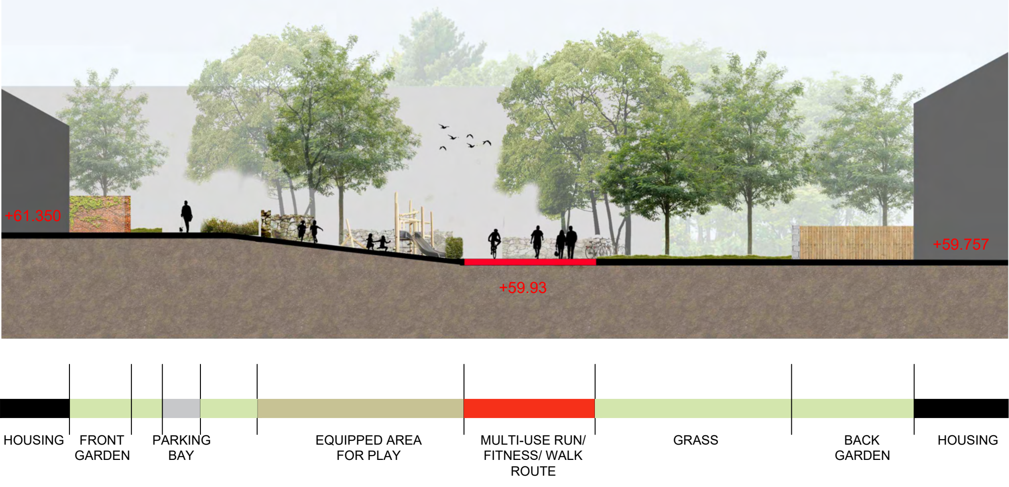
LANDSCAPE SECTION 19-19 sc 1/200
