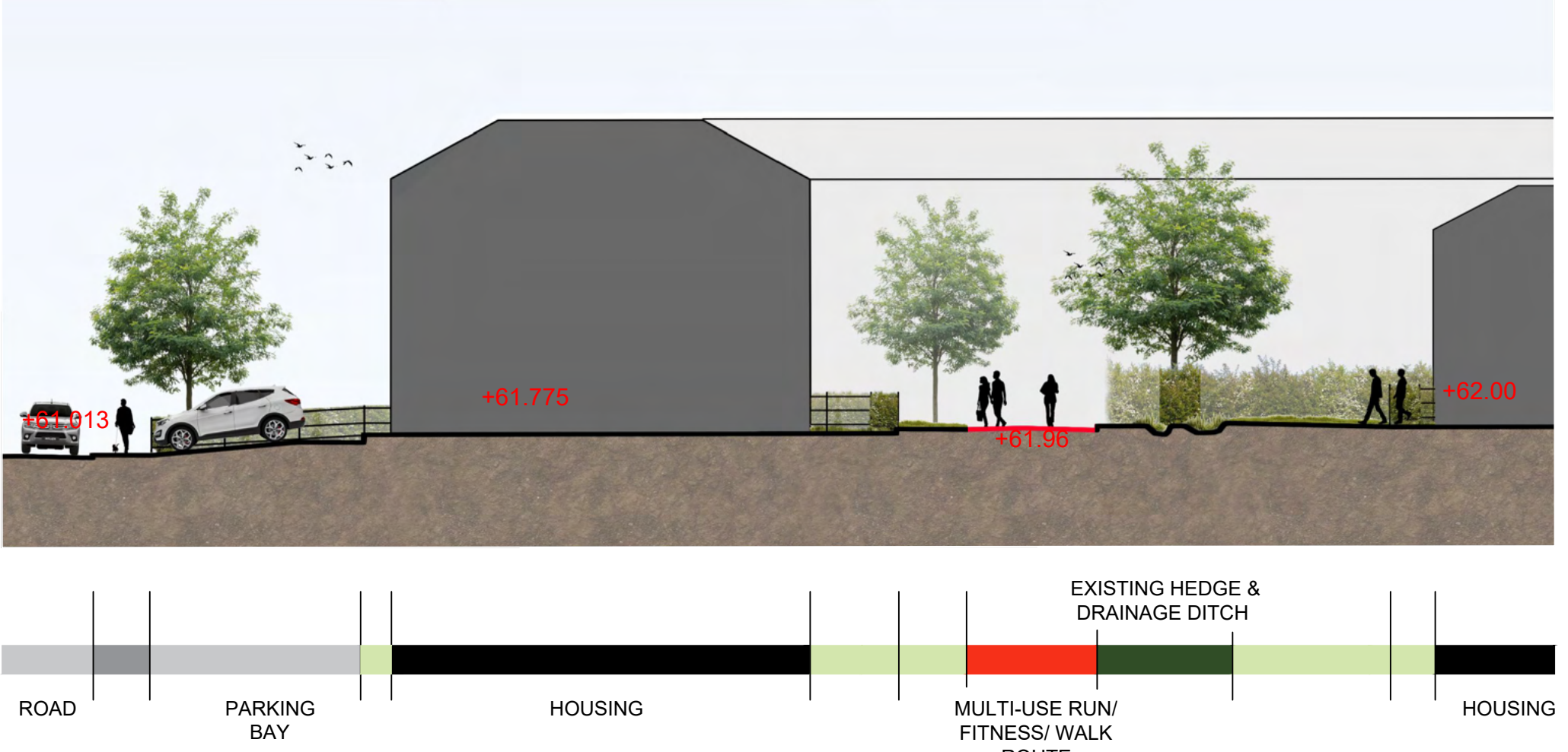
LANDSCAPE SECTION 18-18 sc 1/200
